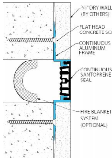
Fire Blanket System (101-A07-050 system shown)
