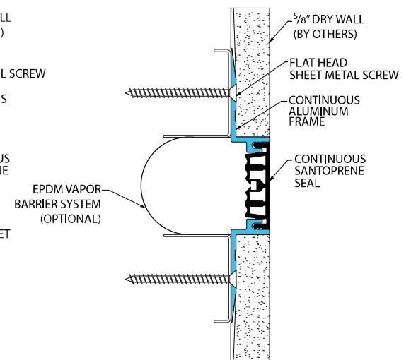
EPDM Vapor Barrier System (101-A07-050 system shown)
