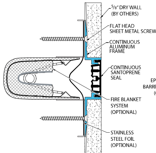
Fire Blanket System (101-A07-050 system shown)
