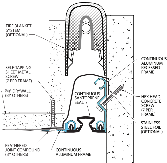
Fire Blanket System (114-A09-050 system shown)
