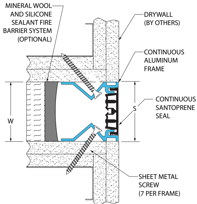
118-A07 Wall/Wall With Mineral Wool (2" (50mm) system shown)
