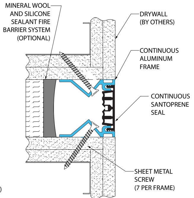
118-A07 Wall/Wall With Mineral Wool (2" (50mm) system shown)
