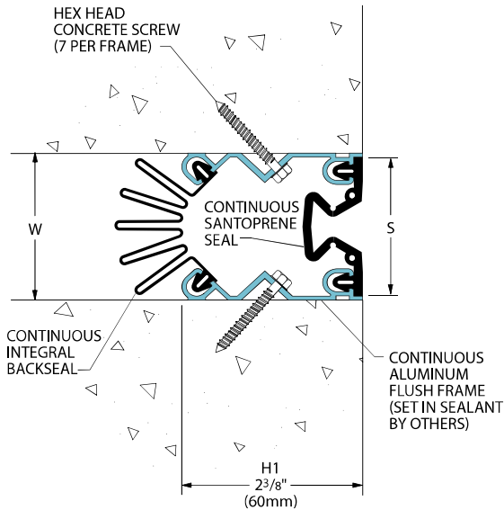
615-A07 Wall/Wall Ceiling/Ceiling (2" (50mm) system shown)
