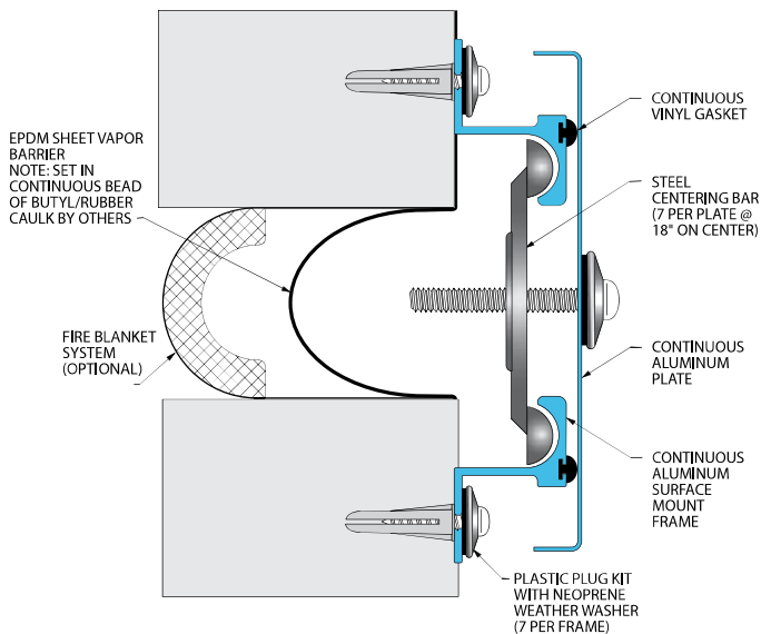
Fire Blanket System (651-A07-050 system shown)
