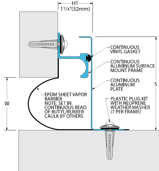
651-A09 Wall/Corner Wall/Ceiling (2" (50mm) system shown)
