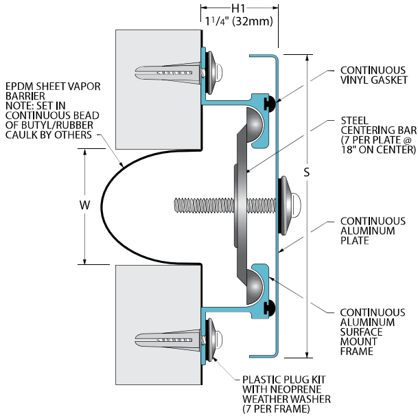
651-A07 Wall/Wall Ceiling/Ceiling (2" (50mm) system shown)
