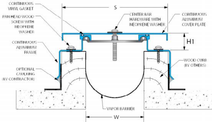
691-A01 Roof/Roof (4" (100mm) system shown)
