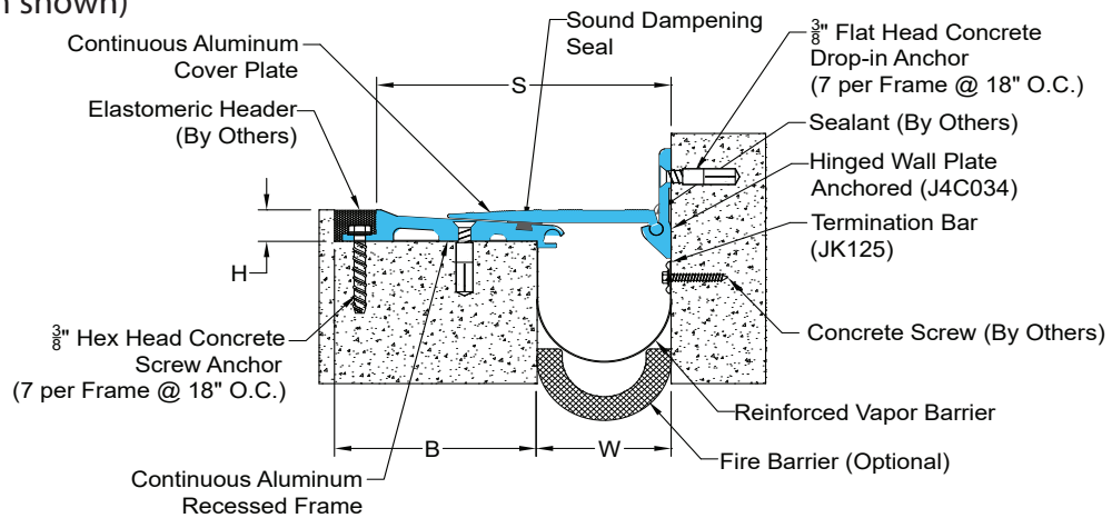
787-A02 Floor/Wall With Vapor Barrier (4" (100mm) system shown)
