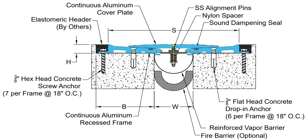
787-A01 Floor/Floor With Vapor Barrier (4" (100mm) system shown)
