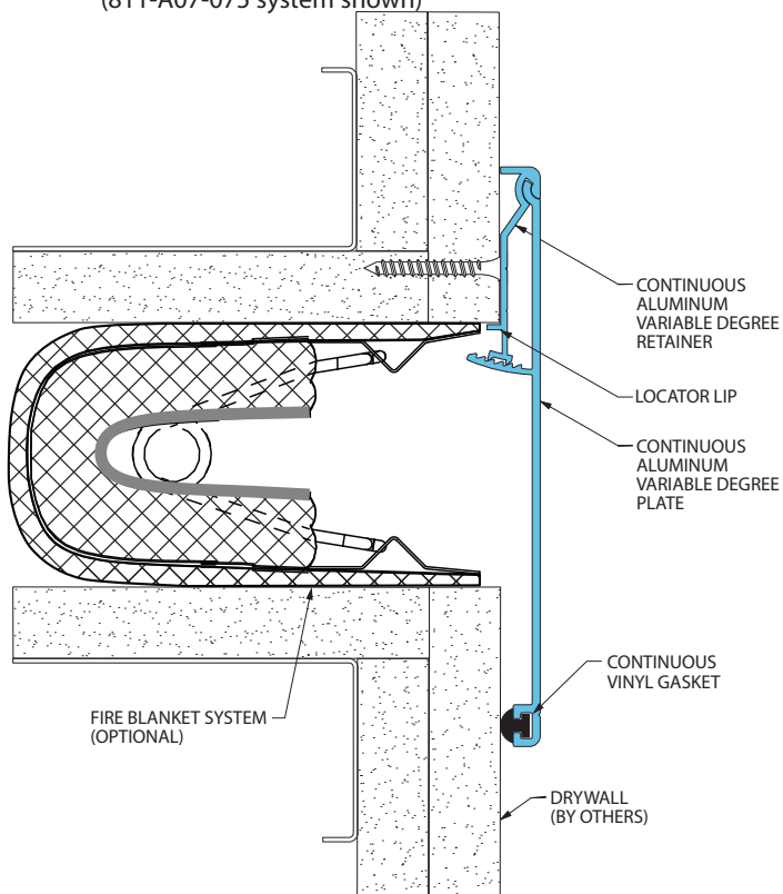
Fire Blanket System (811-A07-075 system shown)
