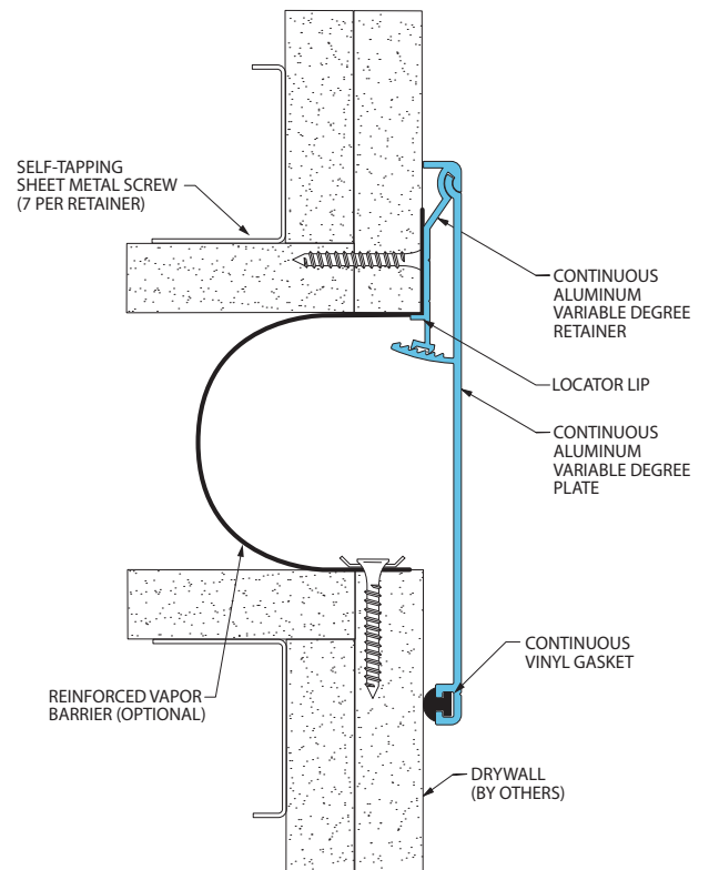
Vapor Barrier System (811-A07-075 system shown)
